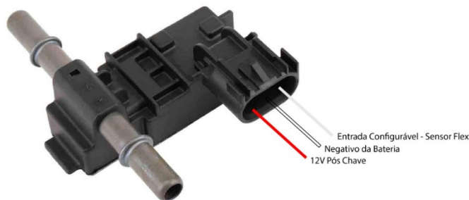
ACDelco 13577429 Sensor Flex Fuel
